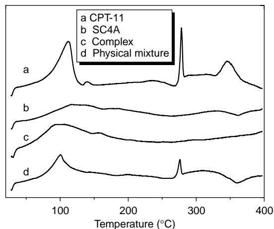
Figure 5. DSC thermograms for (a) CPT-11, (b) SC4A, (c) SC4A-CPT-11 complex and (d) physical mixture (SC4A:CPT-11, 1:1, molar ratio).
