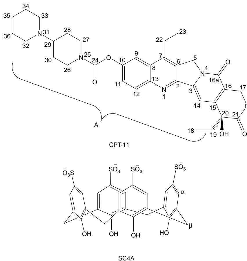
Scheme 1. Chemical structures of CPT-11 and SC4A. Protons of CPT-11 are shown for NMR purposes.
