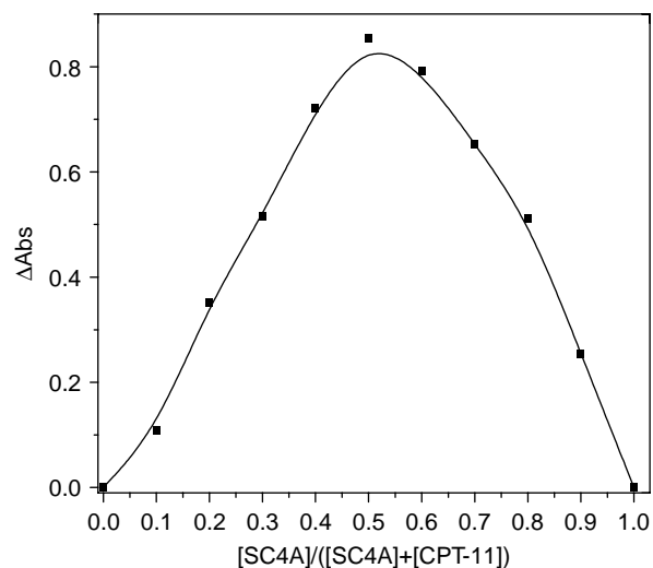
Figure 2. Job plot for SC4A binding of CPT-11. The total concentration was maintained at 0.5 mM and the changes of absorbance were measured at 232 nm.
