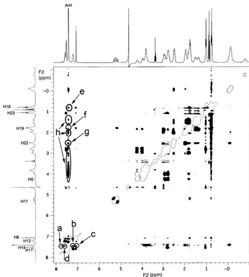
Figure 3. 2D ROESY spectra of SC4A-CPT-11 complex in D_2O . Annotated cross peaks indicate intermolecular interactions between CPT-11 and SC4A.
