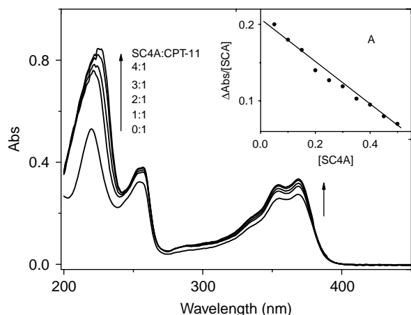
Figure 1. UV spectra of CPT-11 in the absence and presence of SC4A in solution. Concentration of CPT-11: 0.1 mM; concentration of SC4A: 0, 0.1, 0.2, 0.3 and 0.4 mM; A is the curve of absorbance difference at various concentrations of SC4A at 232 nm.
