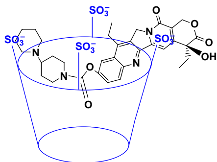
Figure 4. Possible binding mode of SC4A-CPT-11 complex.
